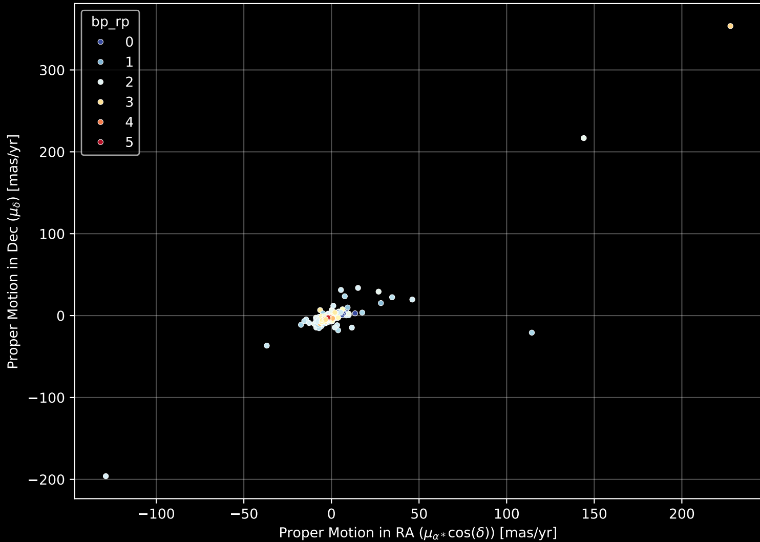
APOGEE DR17 Field: [090+00] Proper Motion Diagram (n= 706)
