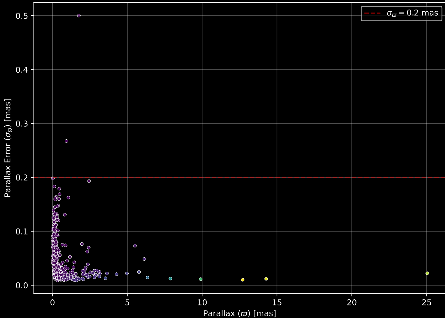
APOGEE DR17 Field: [090+00] Parallax Quality (n= 706)
