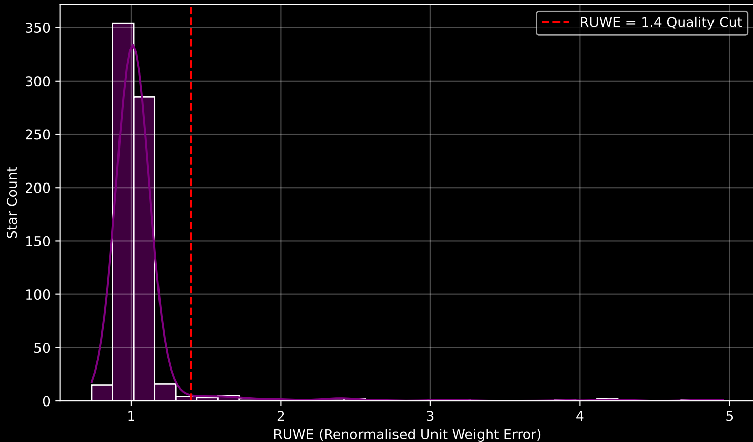
GAPOGEE DR17 Field [090+00] RUWE Distribution (n= 700)
