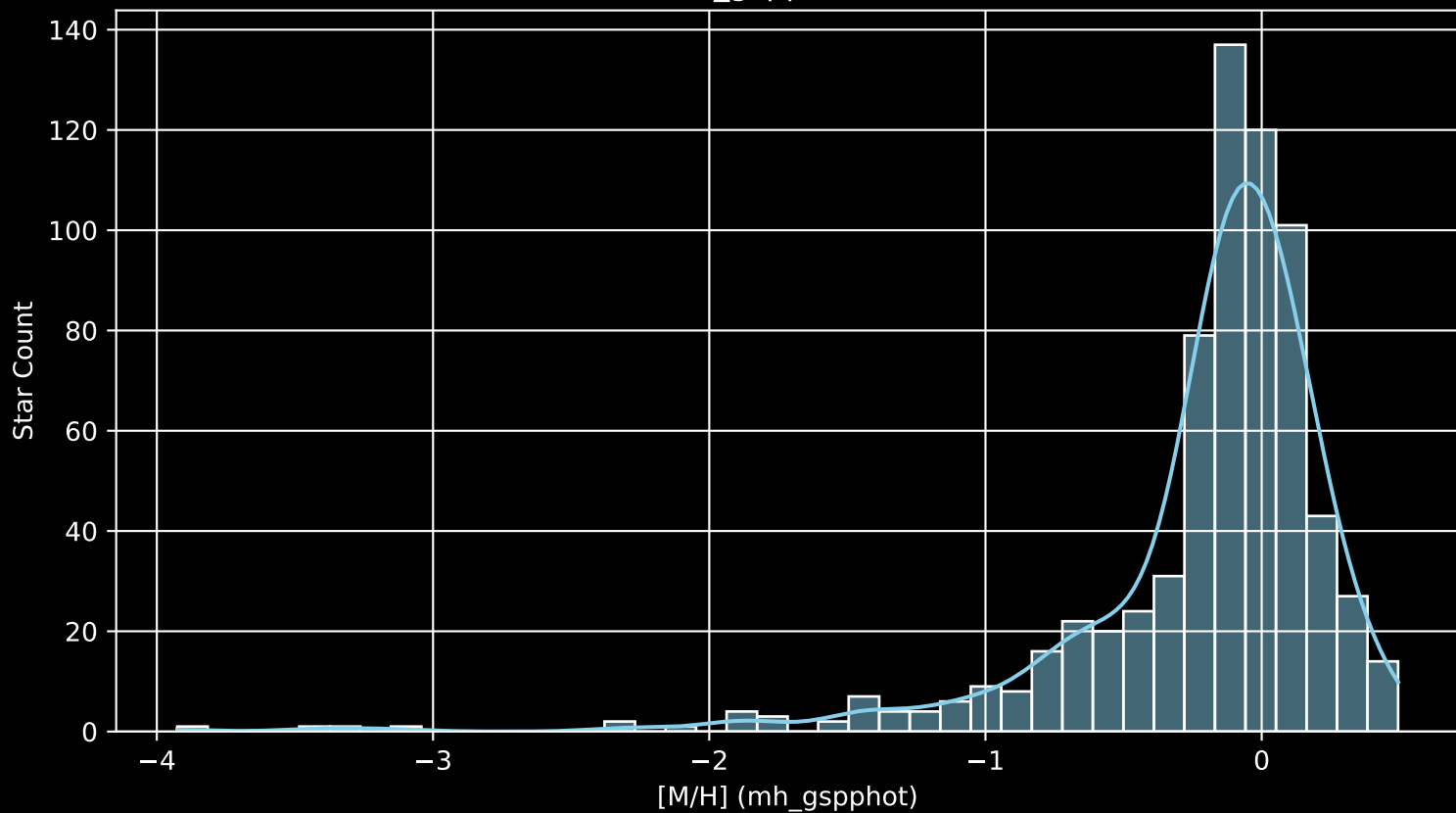
APOGEE DR17 Field: [090+00 [M/H] (mh_gspphot) (n= 688)
