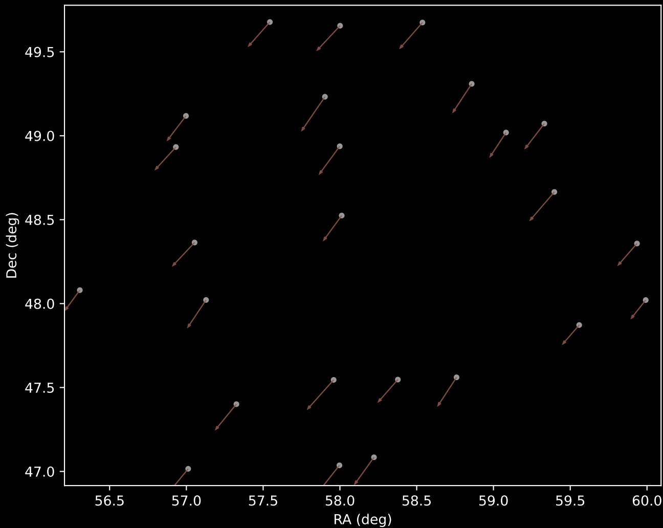
APOGEE DR17 Cluster 30 Proper Motion Vectors (n=25)
