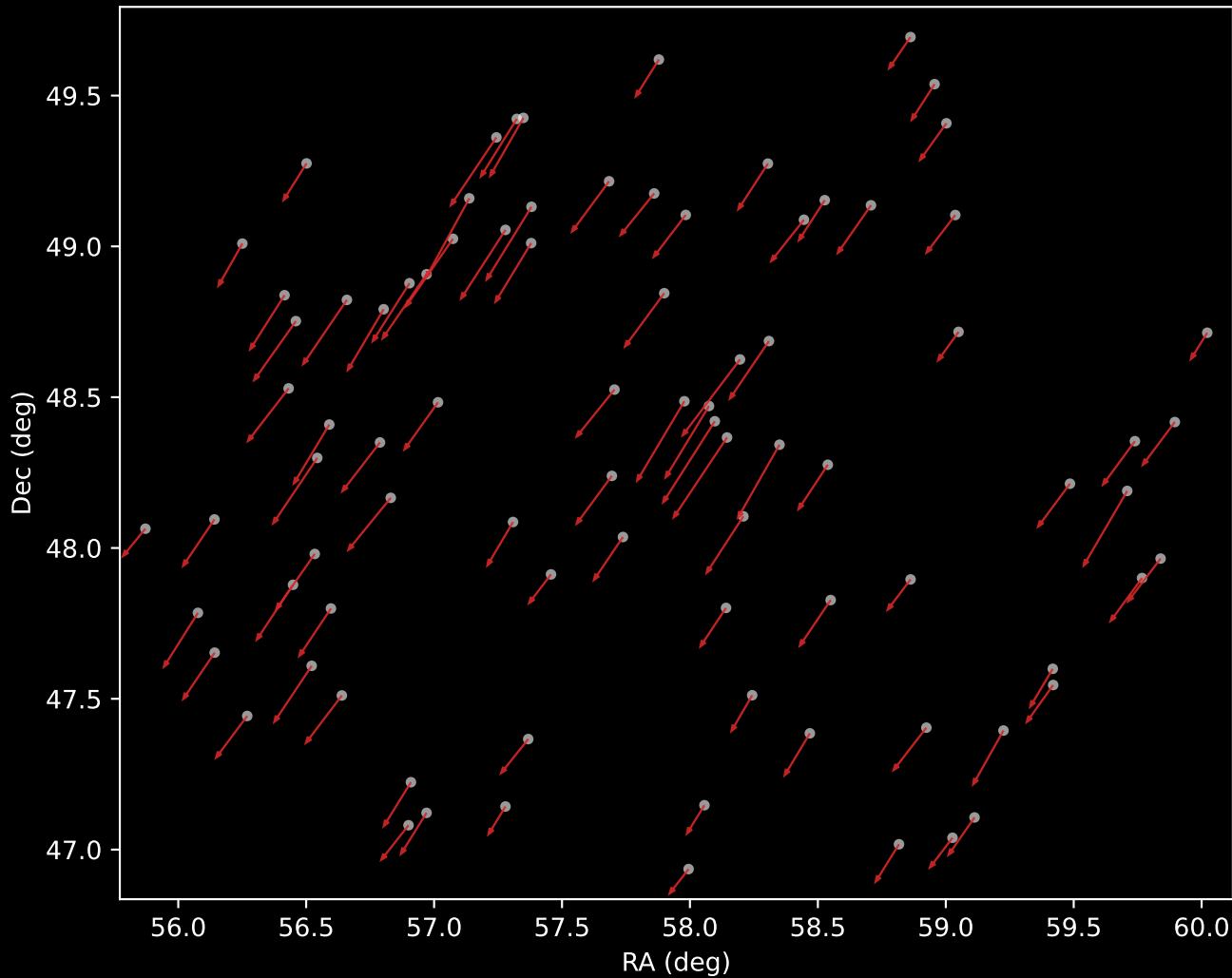
APOGEE DR17 Cluster 26 Proper Motion Vectors (n=86)
