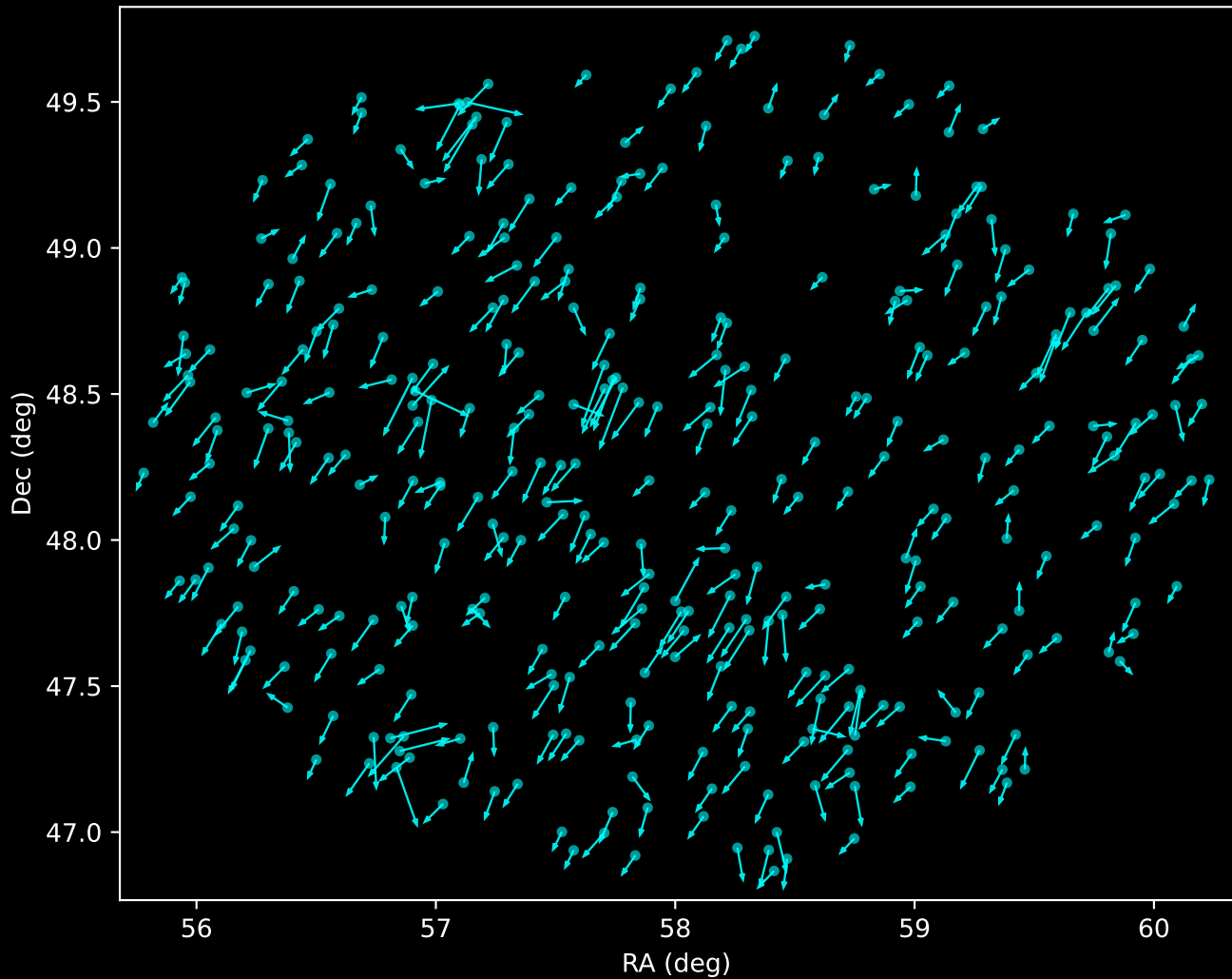
APOGEE DR17 Noise Stream Proper Motion Vectors (n=350)
