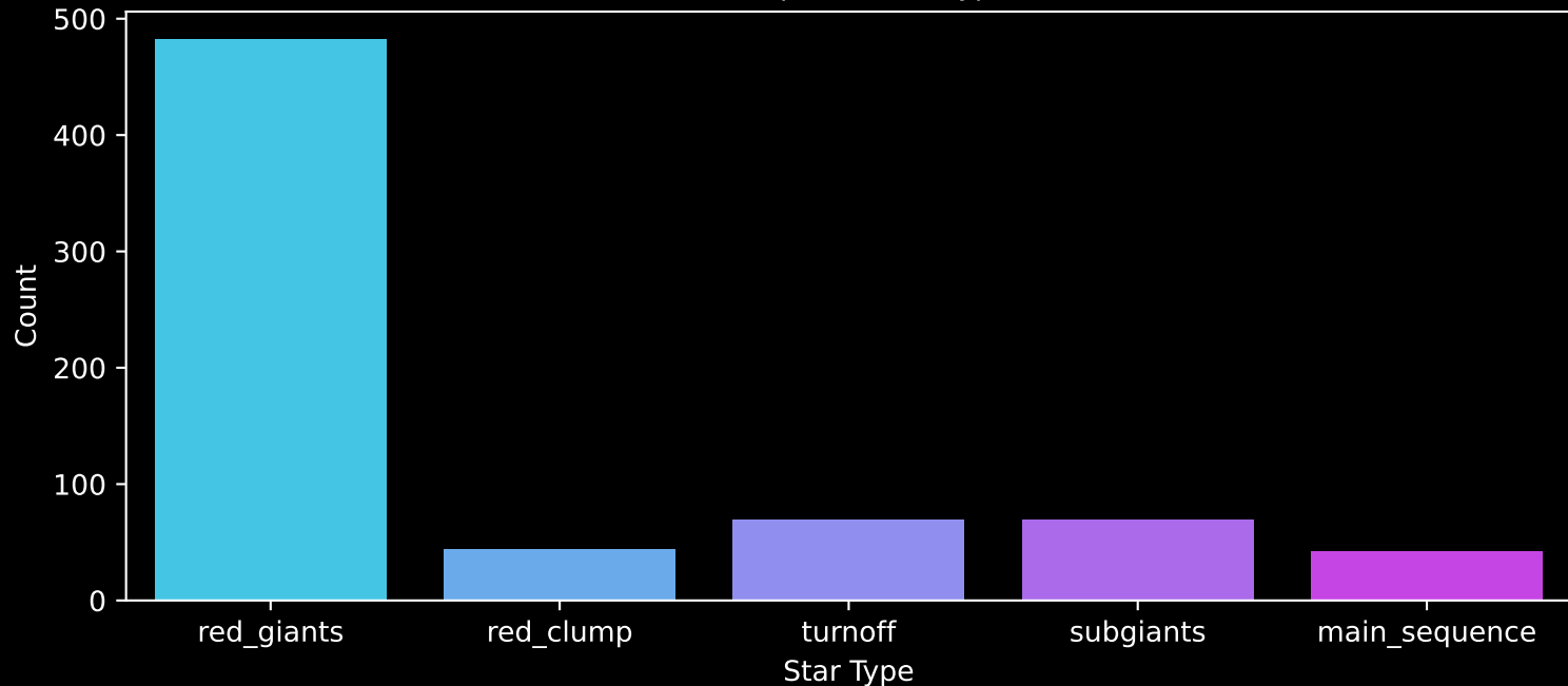
APOGEE DR17 Field: [090+00] Count plot of Star Type
